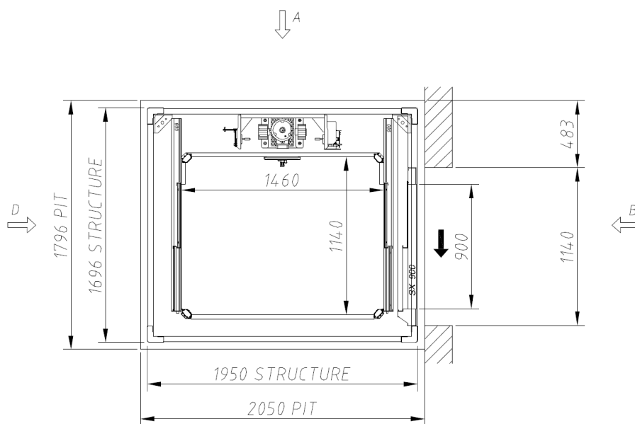
TOP VIEW GROUND FLOOR
