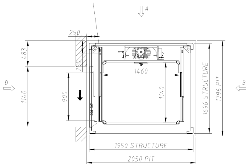
TOP VIEW GROUND FLOOR
