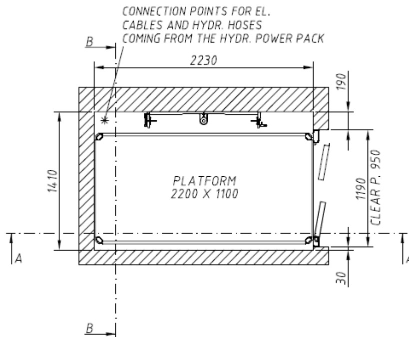
TOP VIEW GROUND FLOOR
